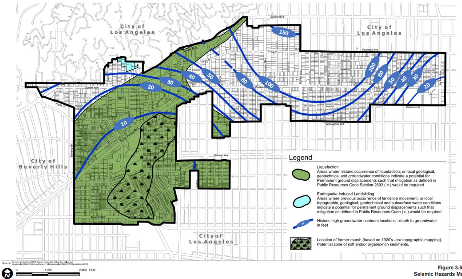
Figure 10. A map depicting the historic high groundwater contours (in blue) with depth to groundwater in feet. The south western portion of the city has the highest water table (at 10 feet), was a former marsh, is prone to liquefaction, and is partially in a 500-year flood FEMA designated zone. This map also depicts regions which are susceptible to seismic induced landslides (light blue). Two areas in the northern portion of the City are given this designation. Source: West Hollywood’s Minimum Prescriptive Foundation Design.
