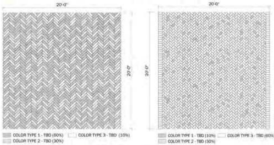
3 Warm gray precast paver colors set in herringbone pattern
